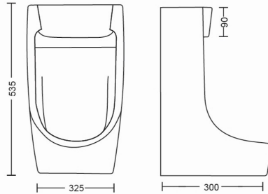
Urinal "Rock" TSB-URN-6015 Size - 300*325*535 (11.8" x 12.7") MRP : 5,900.00
