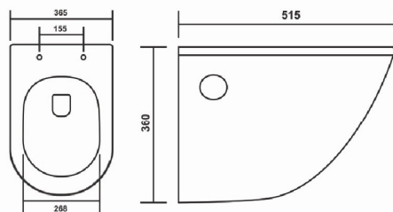
Rimless Wall Hung Toilet "Bravo" TSI-RWH- 5068 Size - 515*365*360 (20") MRP : 8,100.00
